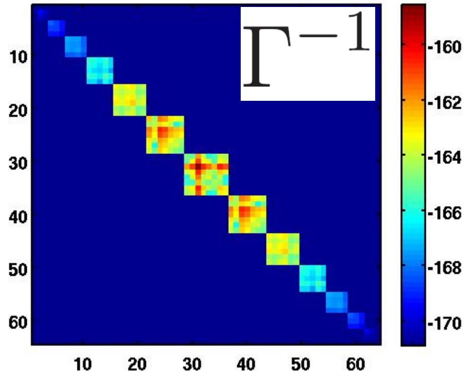
Covariance matrix
