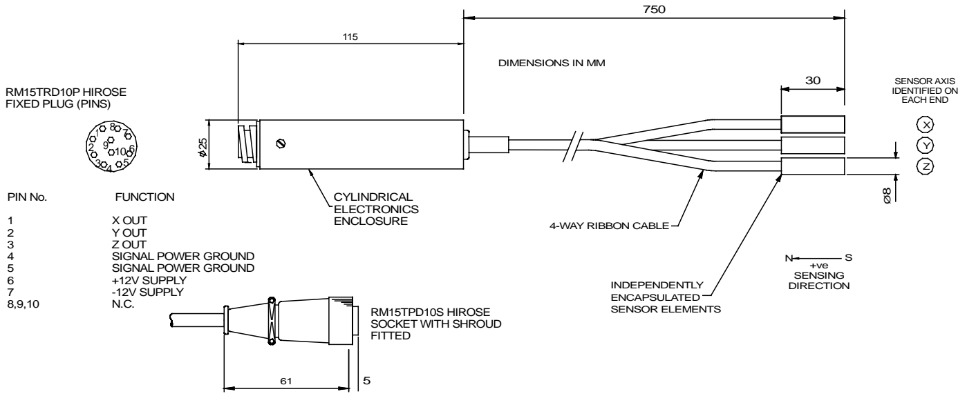
Figure 7 Mag-03IE SENSOR OUTLINE WITH MATING CONNECTOR DR0747(3)
