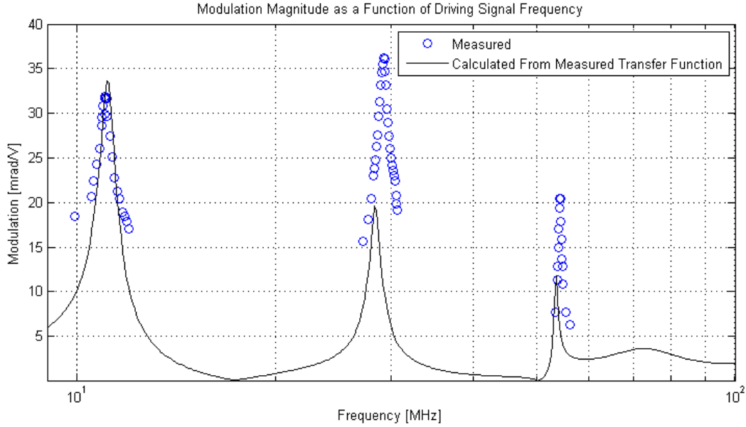
Figure 14: Measured modulation depth as a function of frequency, shown with the expected modulation depth as calculated using the measured transfer function and the nominal modulation depth of the commercially purchased EOM (13 mrad/V)
