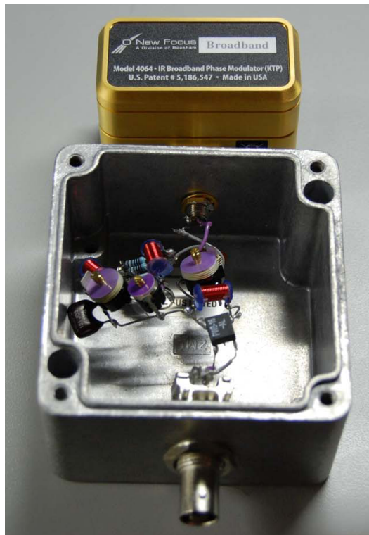
Figure 12: Picture of flying-component circuit in box attached to EOM
