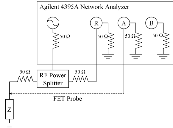
Figure 16: Schematic of impedance testing setup
