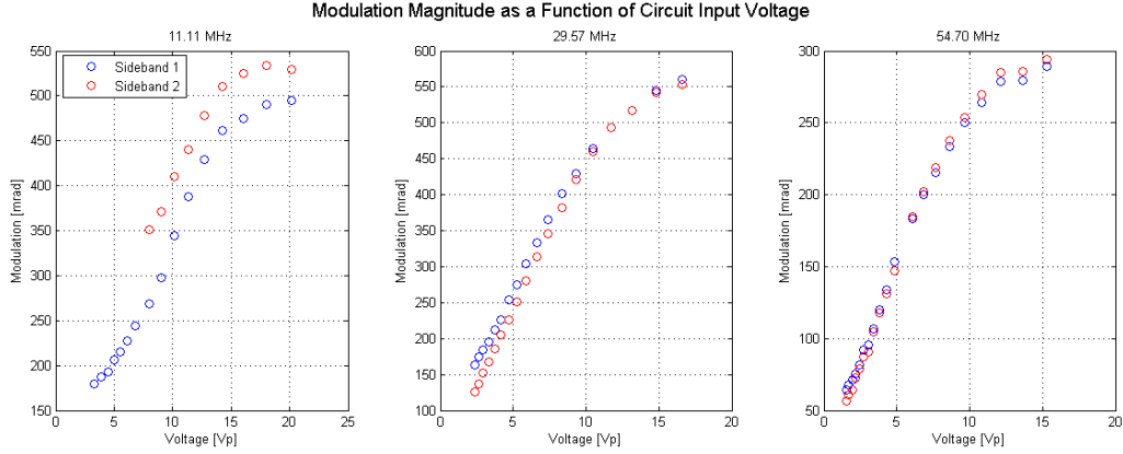
Figure 15: Linear dependance of modulation depth on voltage across input terminals of circuit at each resonant peak (11.11, 29.57, 54.70 MHz)
