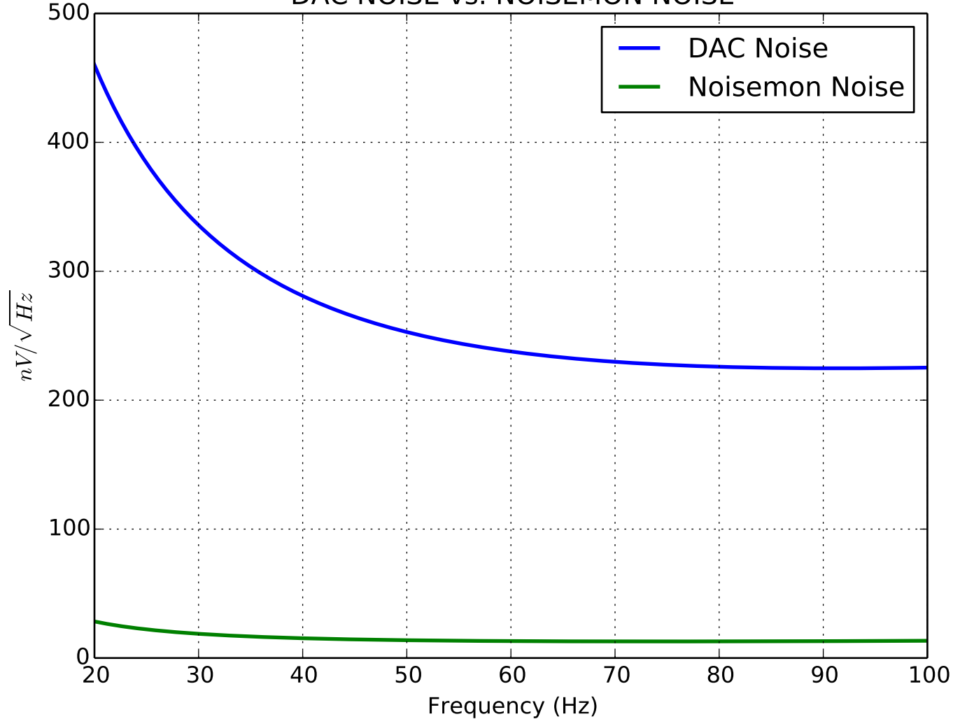
DAC NOISE vs. NOISEMON NOISE
