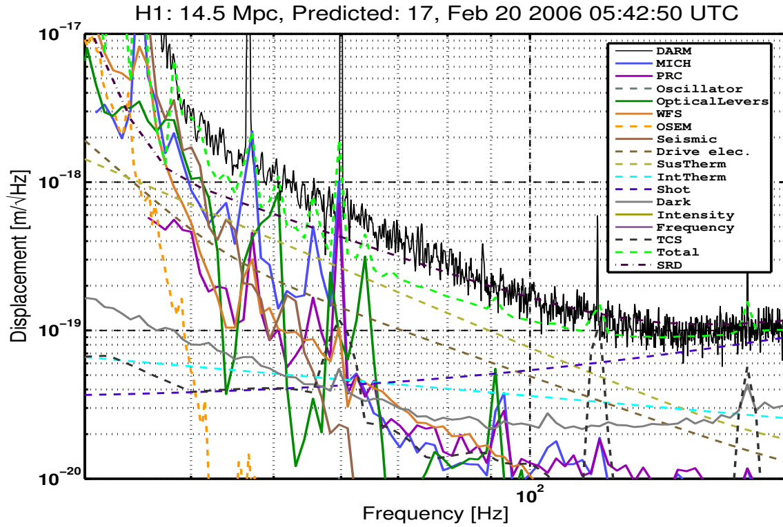
Figure 2-17: H1 Noise Budget (zoom): Zoomed version of figure 2-16. The displacement spectrum is shown in solid black. The incoherent sum of all noise sources is dashed green. See text for more information.
