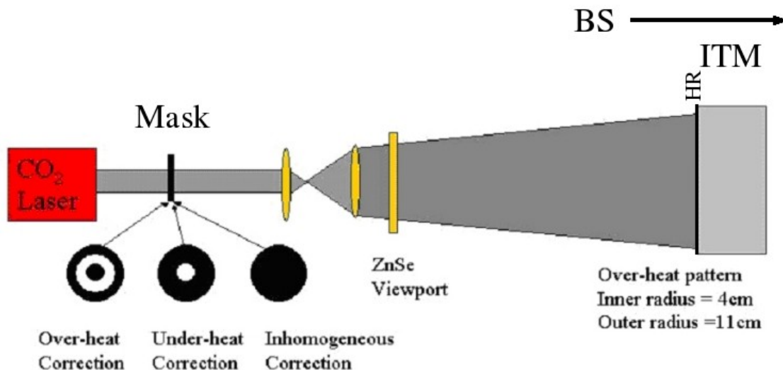
Figure 2-7: A schematic of the Thermal Compensation System (TCS) that was installed on both ITM's on all 3 interferometers. It consists of a 10.6 \mu m CO 2 Laser, a set of masks and a projection system that produces an image of the mask on the optic. See text for more details.
