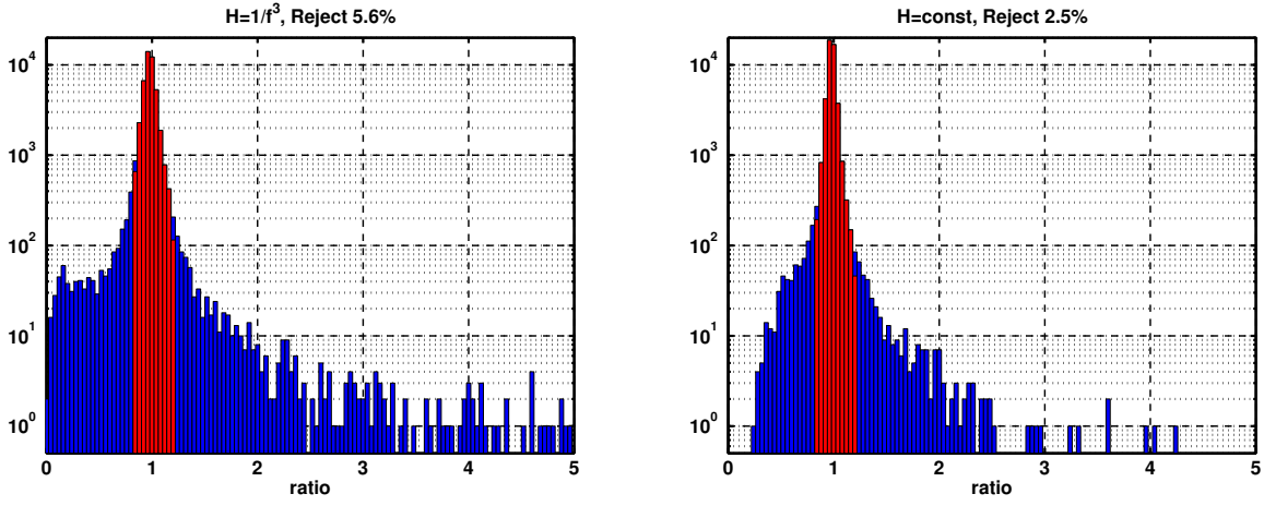
Figure 3-10: Histogram of the ratio \sigma_{\text{middle}}/\sigma_{\text{adjacent}} for the final S4 analysis (see chapter 4). Left for H(f) = \frac{1}{f^3} \text{ Hz}^2 , right for H(f) = 1 \text{ Hz}^{-1} . Blue is before the cut, red after the cut (eq. 3.52).
