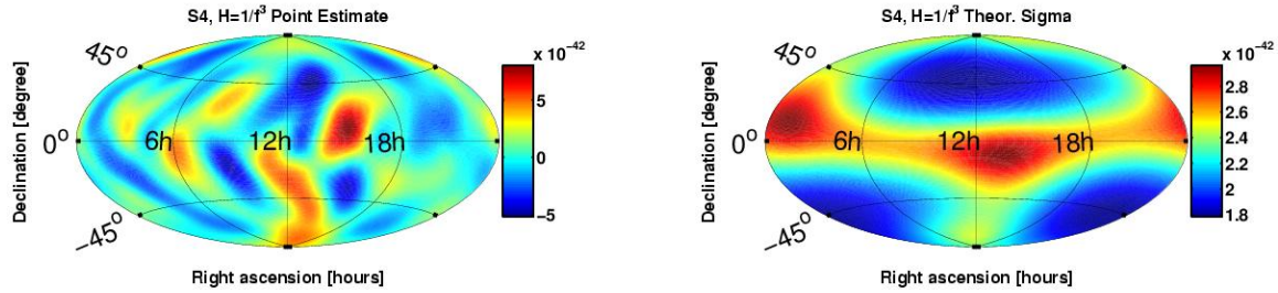
Figure 4-3: S4 Result: Map of the point estimate Y (left) and the theoretical standard deviation \sigma for H(f) = \frac{1}{f^3} \text{Hz}^2 .
