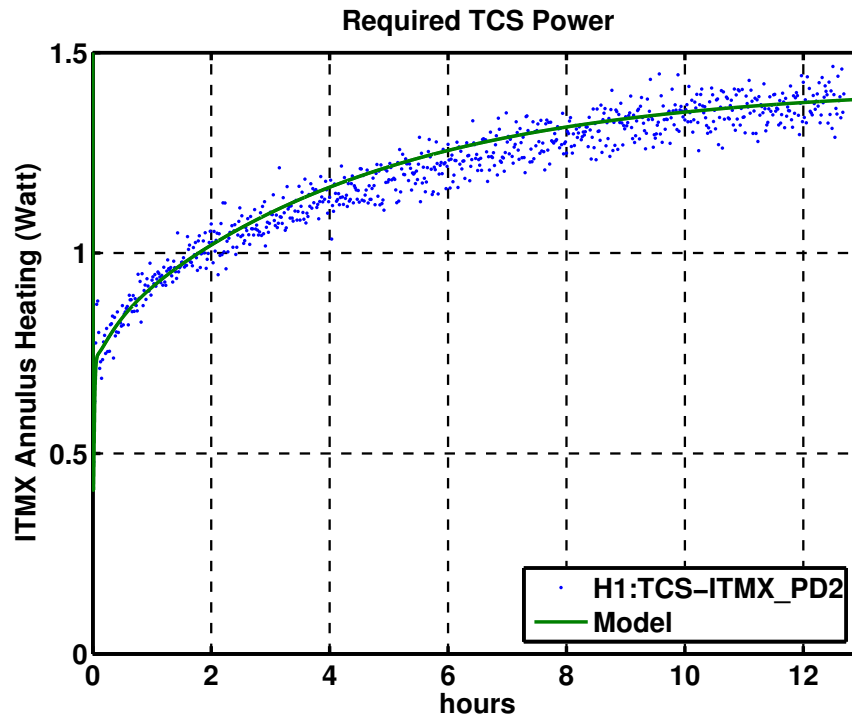
Figure 2-11: Annulus compensation power required to keep the thermal lens constant. The solid green line is calculated as described in the text. The blue dots are photo diode read-backs of the applied compensation power over a 12 hour lock, during which the servo system kept the interferometer at the optimal operations point.
