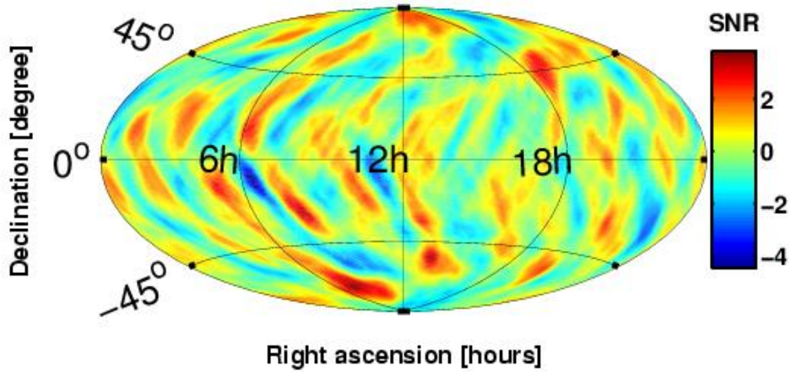
Figure 3-2: An example map of the signal-to-noise ratio \text{SNR} = Y_{\text{opt}}/\sigma_{\text{opt}} for simulated Gaussian noise (see text). The visible structure - fringes with opposite tilt on the northern and southern hemisphere as required by the antipodal symmetry of the antenna lobe - is due to the antenna lobe.
