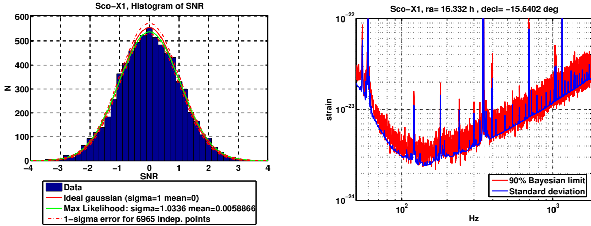
Figure 4-7: S4 Result for Sco-X1: For each 0.25 Hz wide frequency bin a pint estimate and standard deviation is calculated. The resulting SNR is histogrammed on the left side. There are no outliers. The resulting 90% confidence Bayesian upper limit as a function of frequency - marginalized over the calibration uncertainty, is plotted on the right (red). Also shown is the standard deviation (blue).
