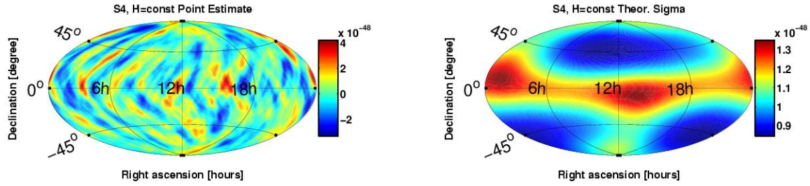
Figure 4-6: S4 Result: Map of the point estimate Y (left) and the theoretical standard deviation \sigma for H(f) = 1 \text{ Hz}^{-1} .
